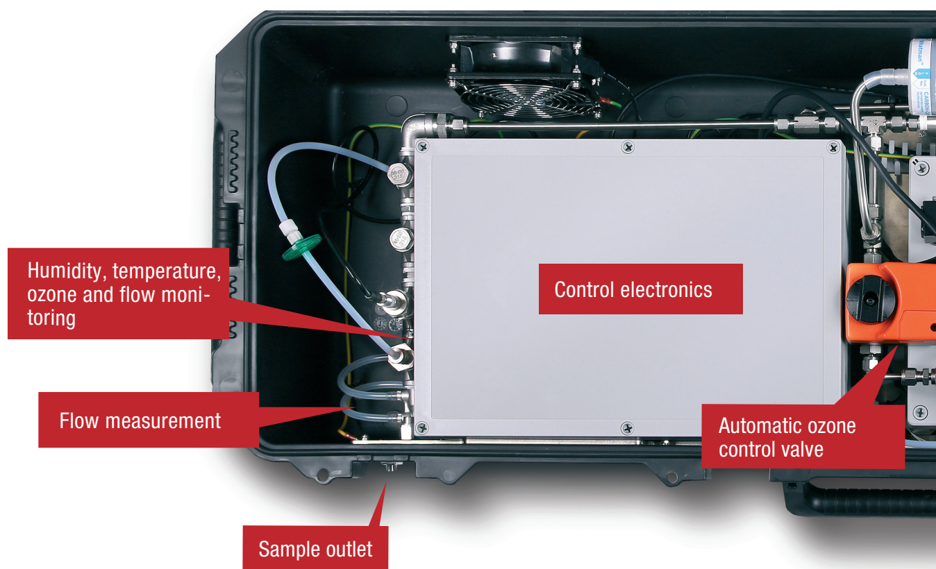
DOFR™ Sample conditioning unit, main components
