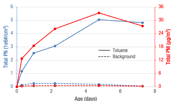
Study of the potential aerosol mass (PAM) of a Toluene precursor as function of the Dekati® DOFR™ equivalent ageing time. Concentrations measured with the Dekati® HR-ELPI®+
