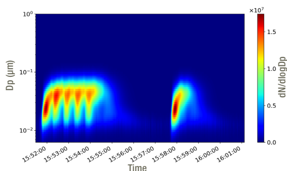
Study of an SOA formation event with rapid Toluene vapor injections. Real-time distribution measured with the Dekati® HR-ELPI®+
