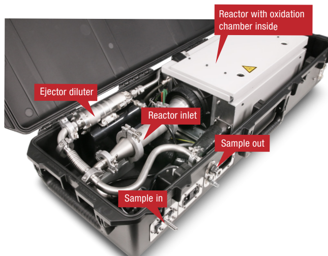
The DOFR™ system is built into a portable casing.
