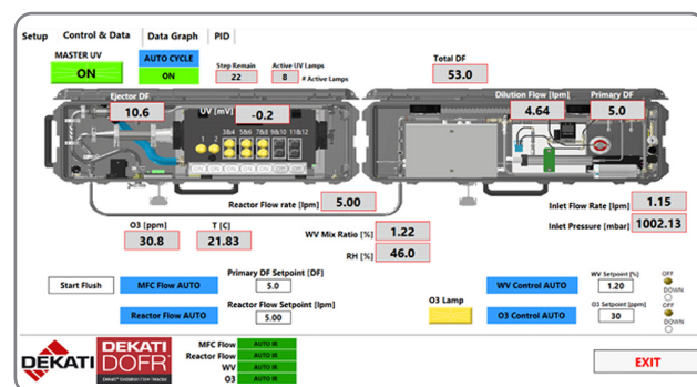
The comprehensive PC user interface of the DOFR™ ensures easy control and monitoring of all main system parameters
